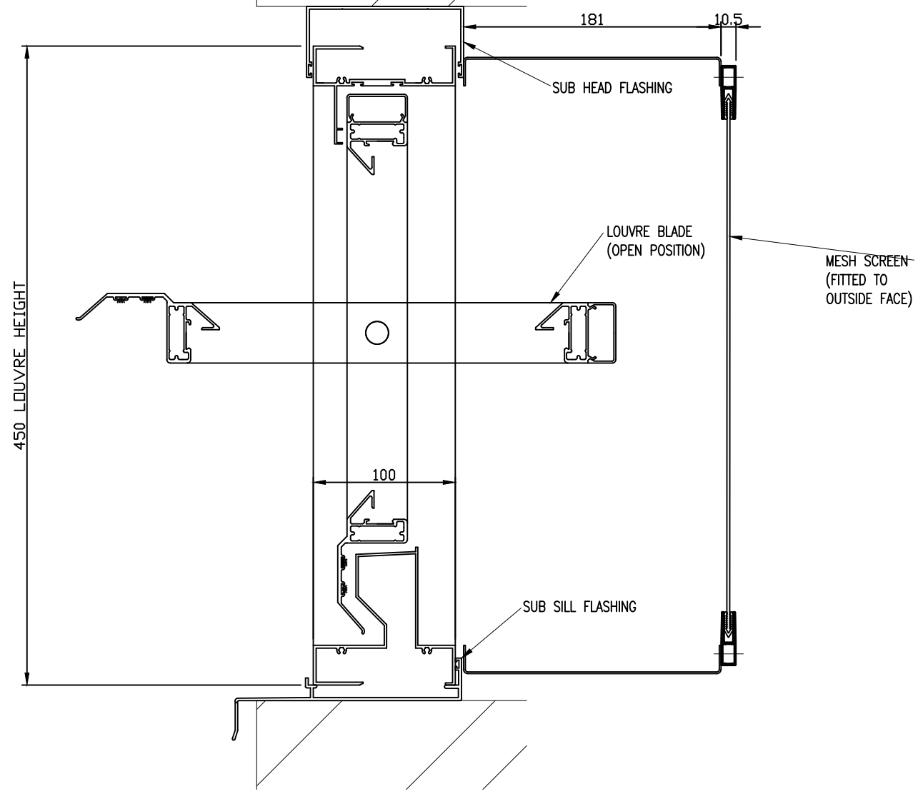
ALUMINIUM STORMGLAZE LOUVRE TYPICAL SECTION DETAIL (WITH EXTERNAL MESH SCREEN)
