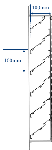
SECTIONAL ELEVATION
