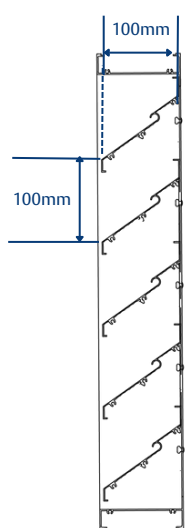
SECTIONAL ELEVATION
