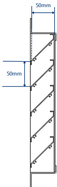
SECTIONAL ELEVATION
