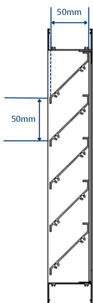
SECTIONAL ELEVATION
