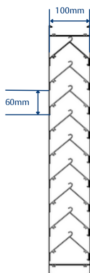
SECTIONAL ELEVATION
