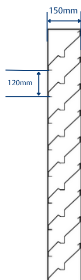
SECTIONAL ELEVATION
