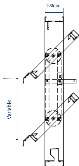
SECTIONAL ELEVATION
